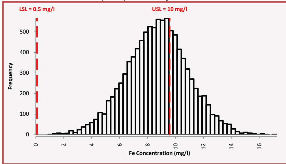
Fig 1: Frequency distribution for Fe concentration (mg/l)
